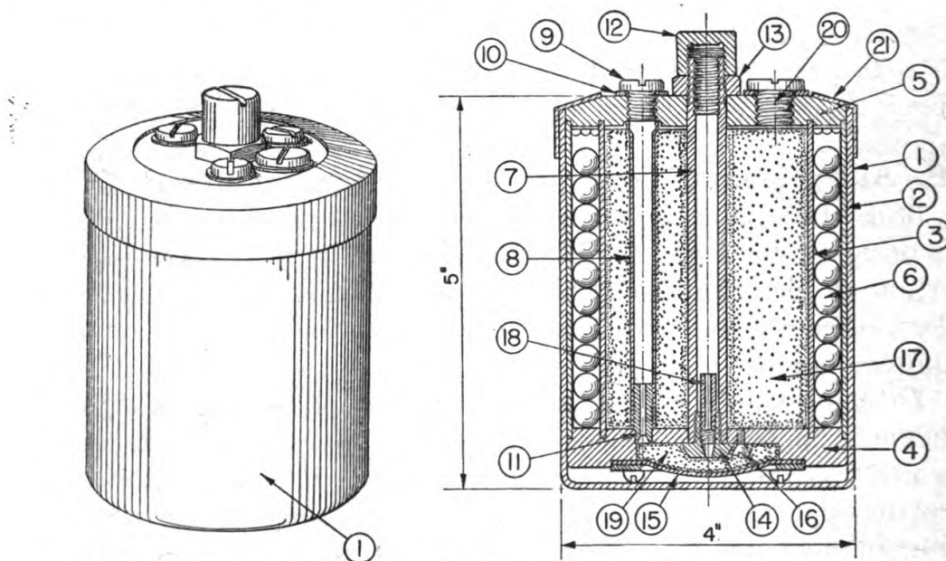
FIGURE 37.—Section and perspective view of antipersonnel bounding mine (silent soldier).
